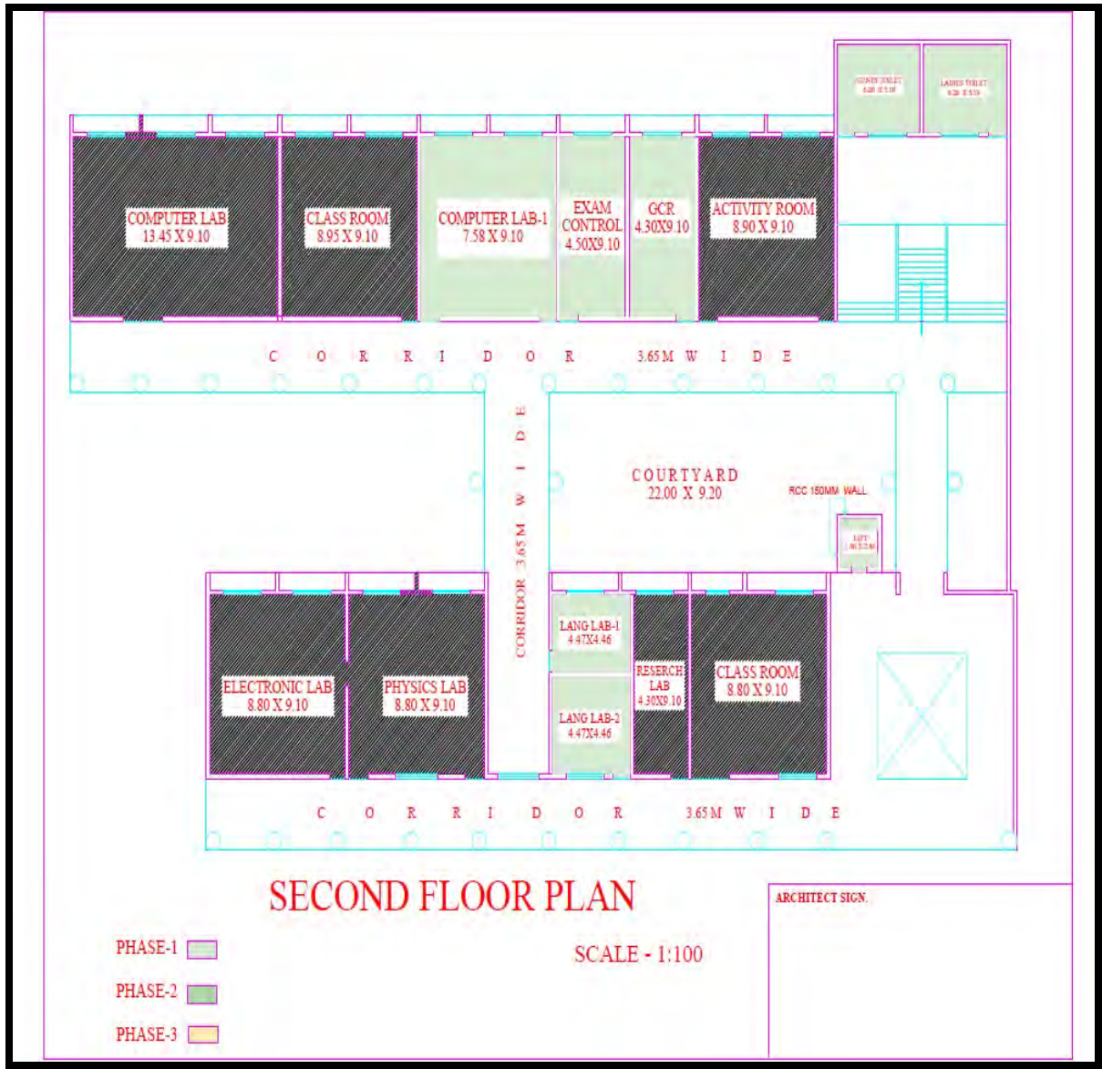
Institute Second Floor Plan
