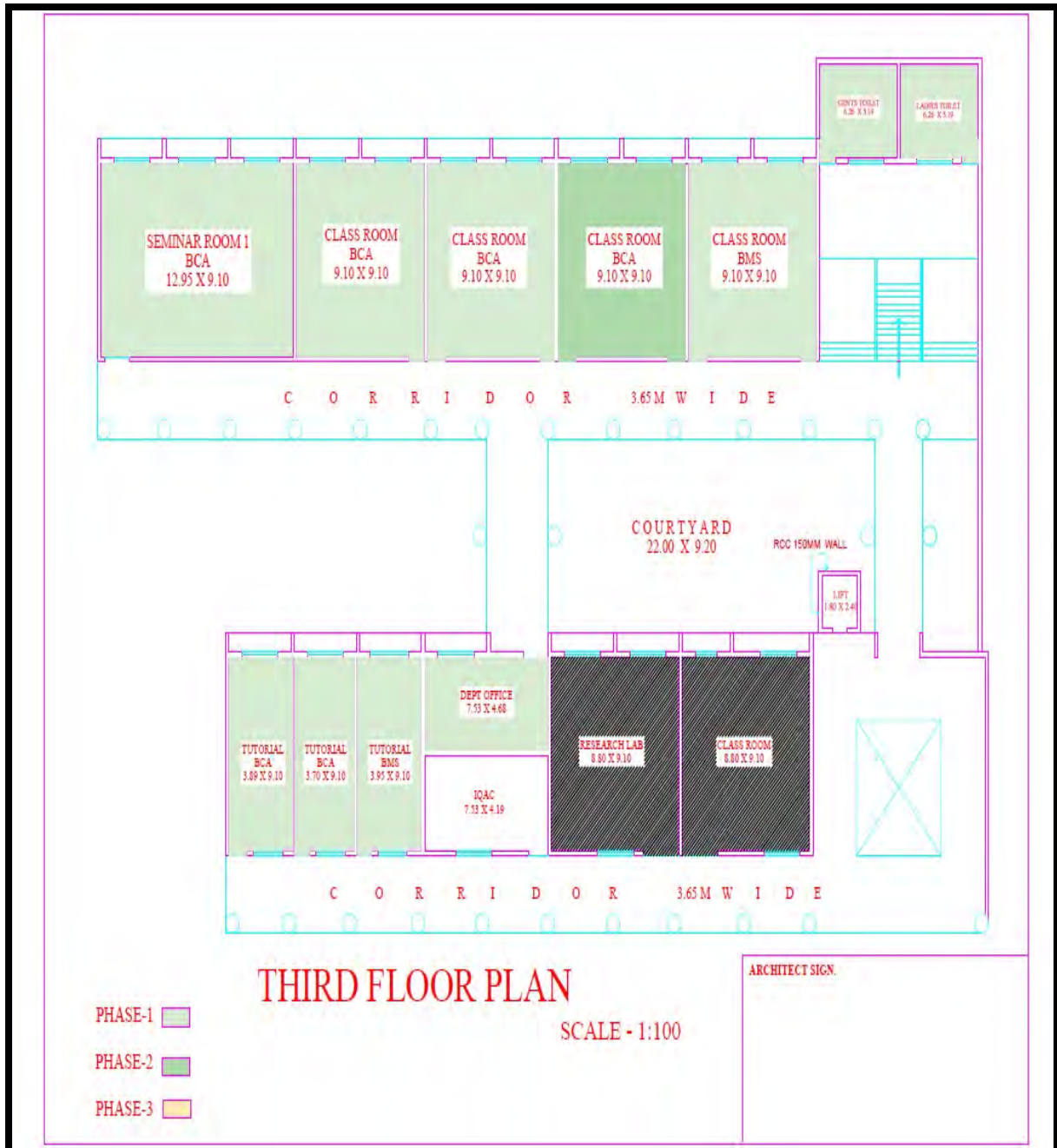
Institute Third Floor Plan
