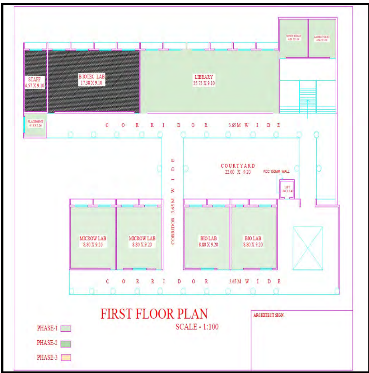
Institute First Floor Plan
